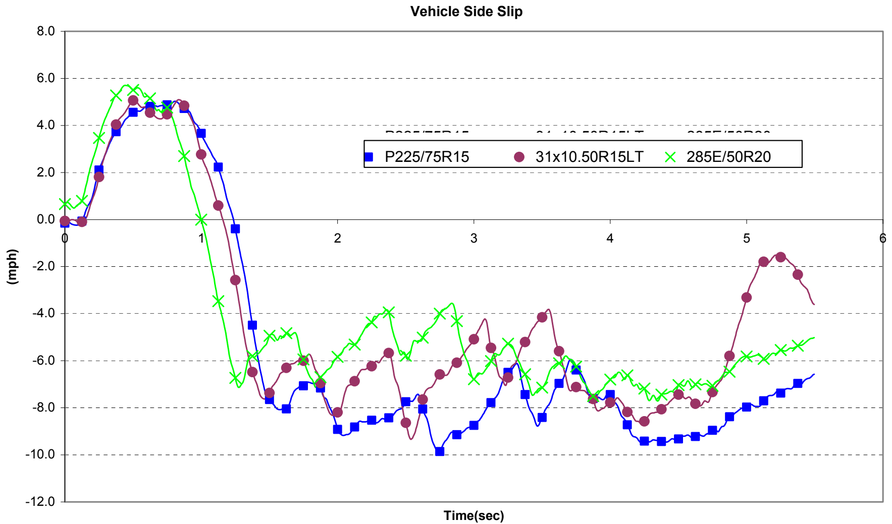
FIGURE 5. Vehicle side slip angles for wheels at near-zero offset. Note that the side slip angle decreases with tire size.
